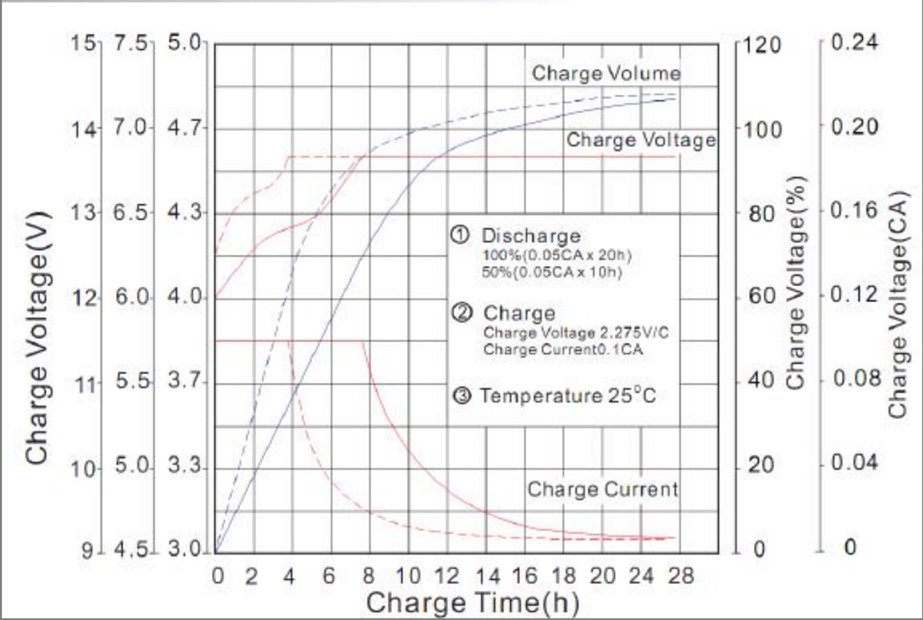
Charge characteristic Curve for standby use
