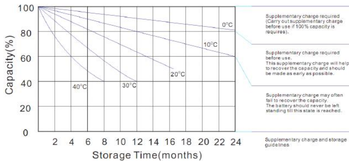
Storage characteristics
