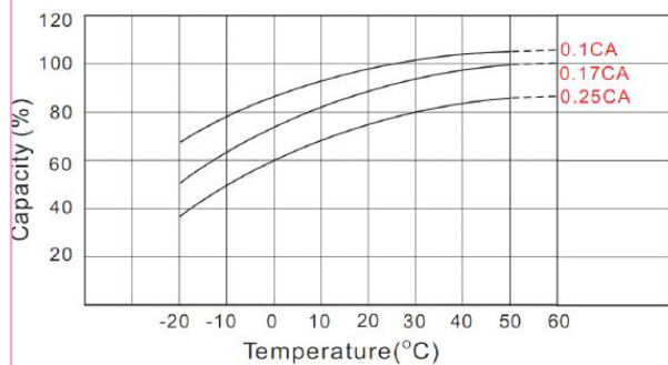
Temperature Effects in Relation to Battery Capacity
